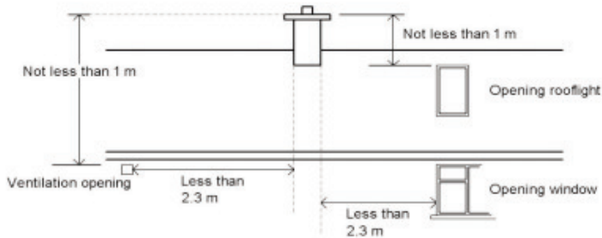
(b) HEIGHT OF FLUE OVER OPENINGS
